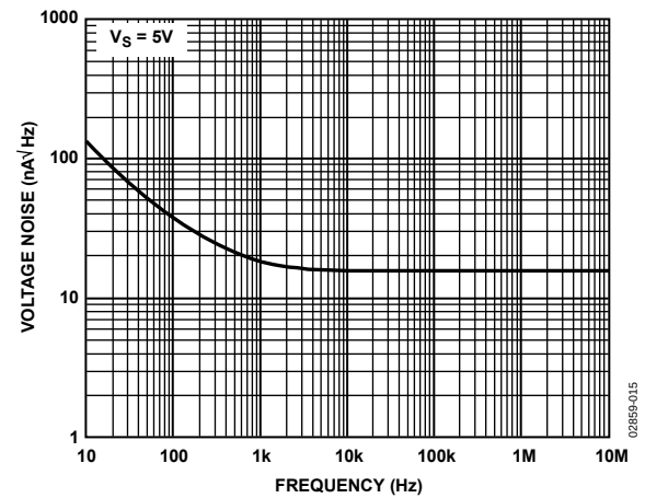
Figure 15. Input Voltage Noise vs. Frequency
